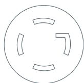
Power cord with plug (NEMA L16-30P twist lock; 30 A)
