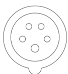
Power cord with plug (IEC 60309, 5-pol, CEE, red, 16 A)
