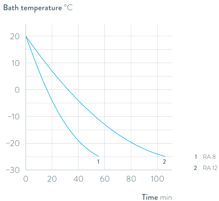
Fig. 10: Alpha cooling curves
