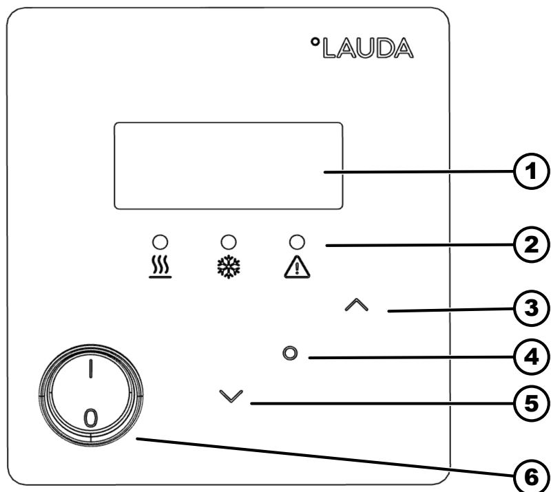
Fig. 3: Control panel
