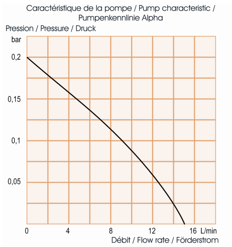
Fig. 11: Alpha pump characteristics
